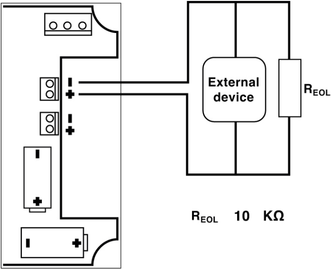
Wiring example for the 12Vdc/24Vdc output.
