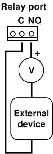
Wiring example for the relay switch output.
